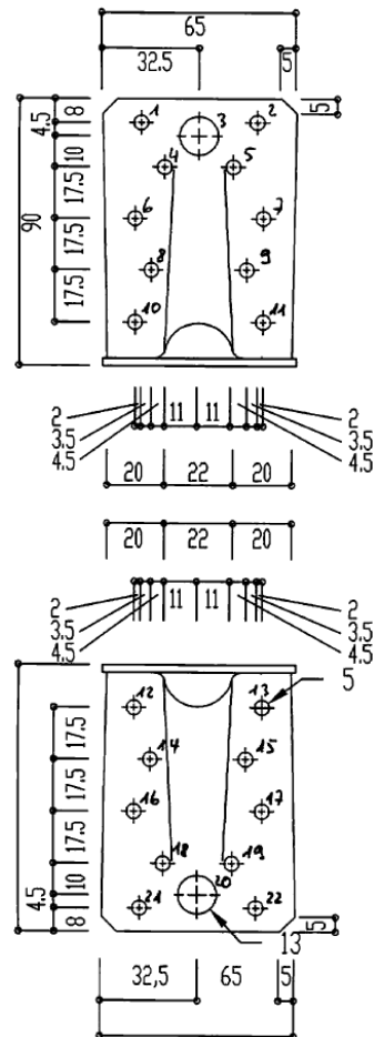
Figure A. 4 Dimensions of Angle Bracket 1112
