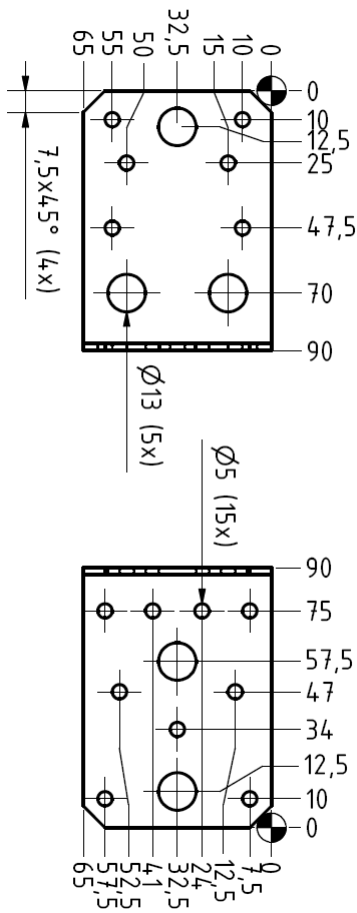
Figure A. 3 Dimensions of Angle Bracket 1132
