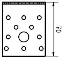
Figure A. 1 Dimensions of Angle Bracket 1131
